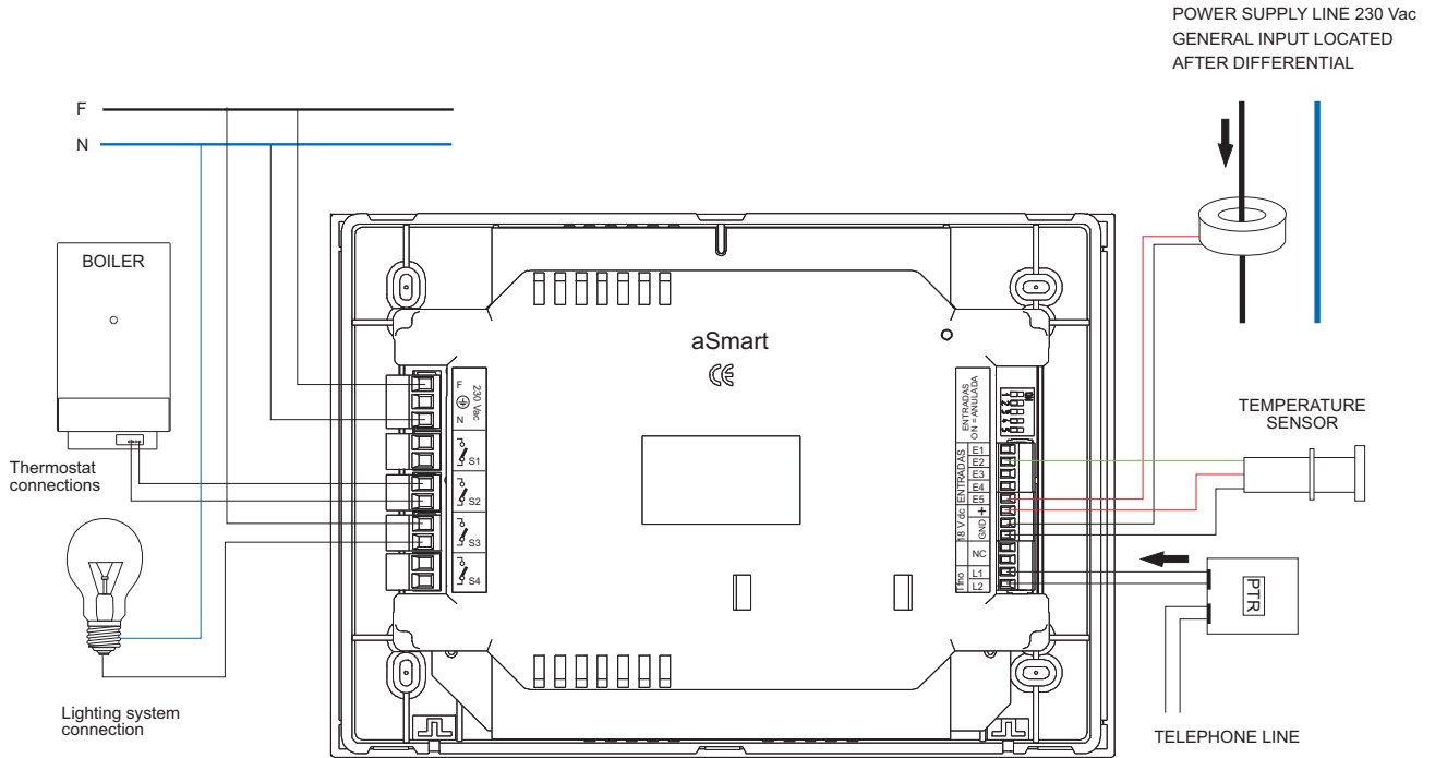
Basic installation schema
